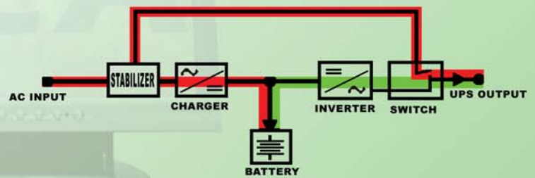
UPS DIAGRAM
